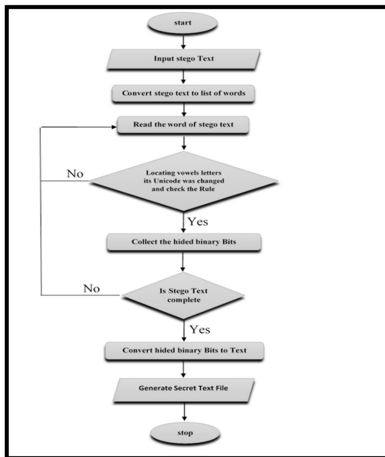
Figure 3 flowchart for Extraction Algorithm 2
